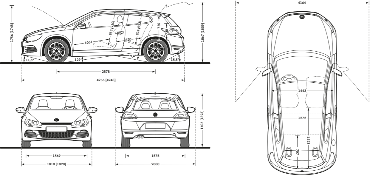
All figures in millimetres. On illustrations, where arrows and figures are shown inside of the vehicle, the measurements are for interior dimensions. Where arrows and figures are shown outside of the vehicle, the measurements are for exterior dimensions.
