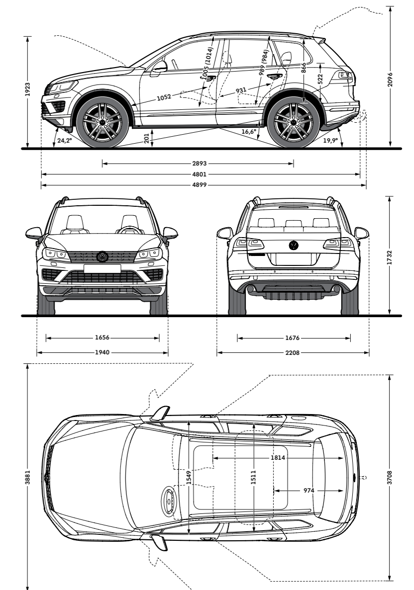
All figures in millimetres. On illustrations, where arrows and figures are shown inside of the vehicle, the measurements are for interior dimensions. Where arrows and figures are shown outside of the vehicle, the measurements are for exterior dimensions.
